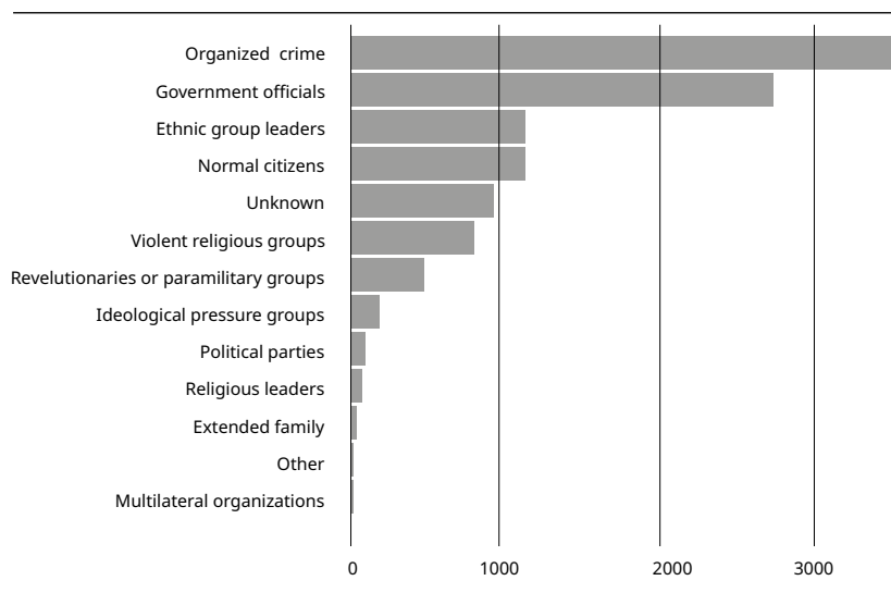
Figure 1. Incident categorized ( 2015 - 2024 )
